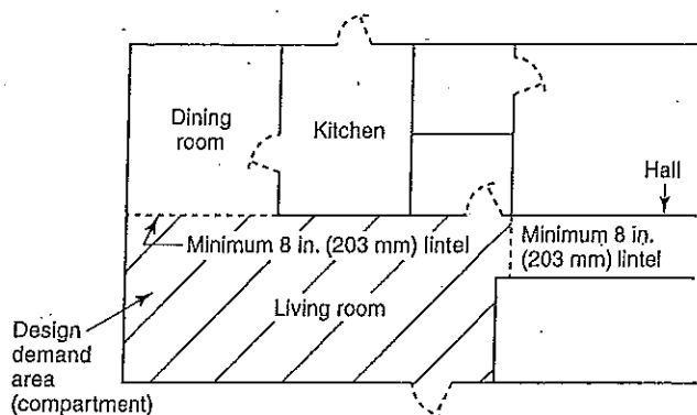
FIGURE A.8.1.2(b) Sprinkler Design Areas for Typical Residential Occupancy — With Lintel.
