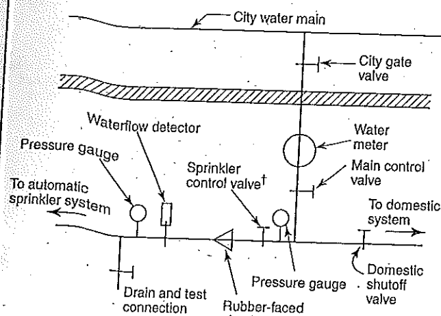
FIGURE A.6.2(b) Acceptable Arrangement for Stand-Alone Piping Systems with Valve Supervision — Option 1.
