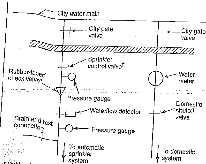
FIGURE A.6.2(b) Acceptable Arrangement for Stand-Alone Piping Systems with Valve Supervision — Option 1.
