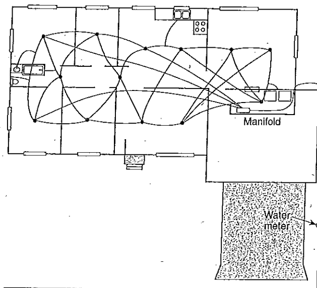
FIGURE A.3.3.9.4 Network System.
