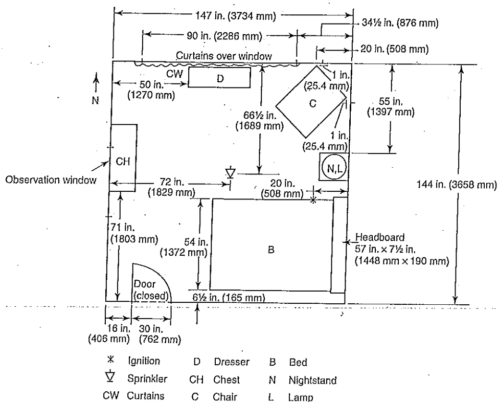
FIGURE A.1.1(a) Bedroom.
