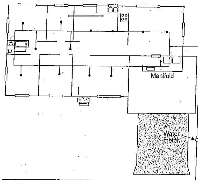
FIGURE A.3.3.9.3(b) Multipurpose Piping System — Example 2.
