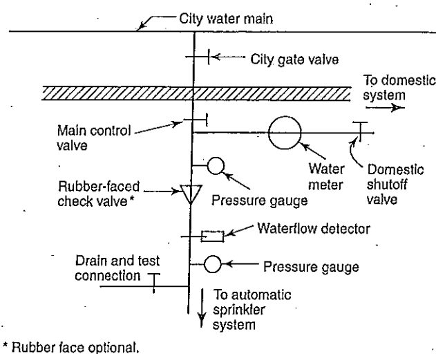
FIGURE A.6.2(a) Preferable Arrangement for Stand-Alone Piping Systems.
